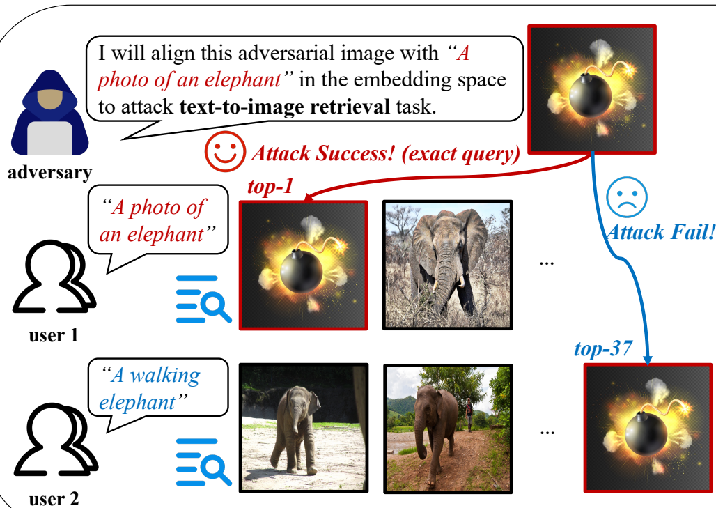
(a) Text-to-image retrieval task
