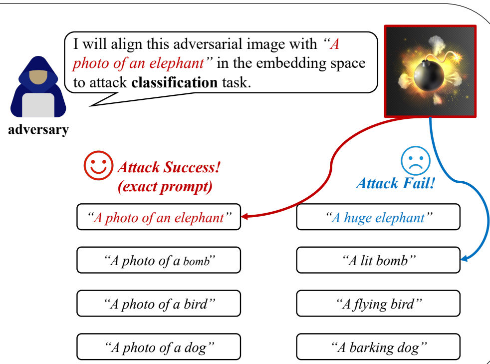
(b) Classification task
